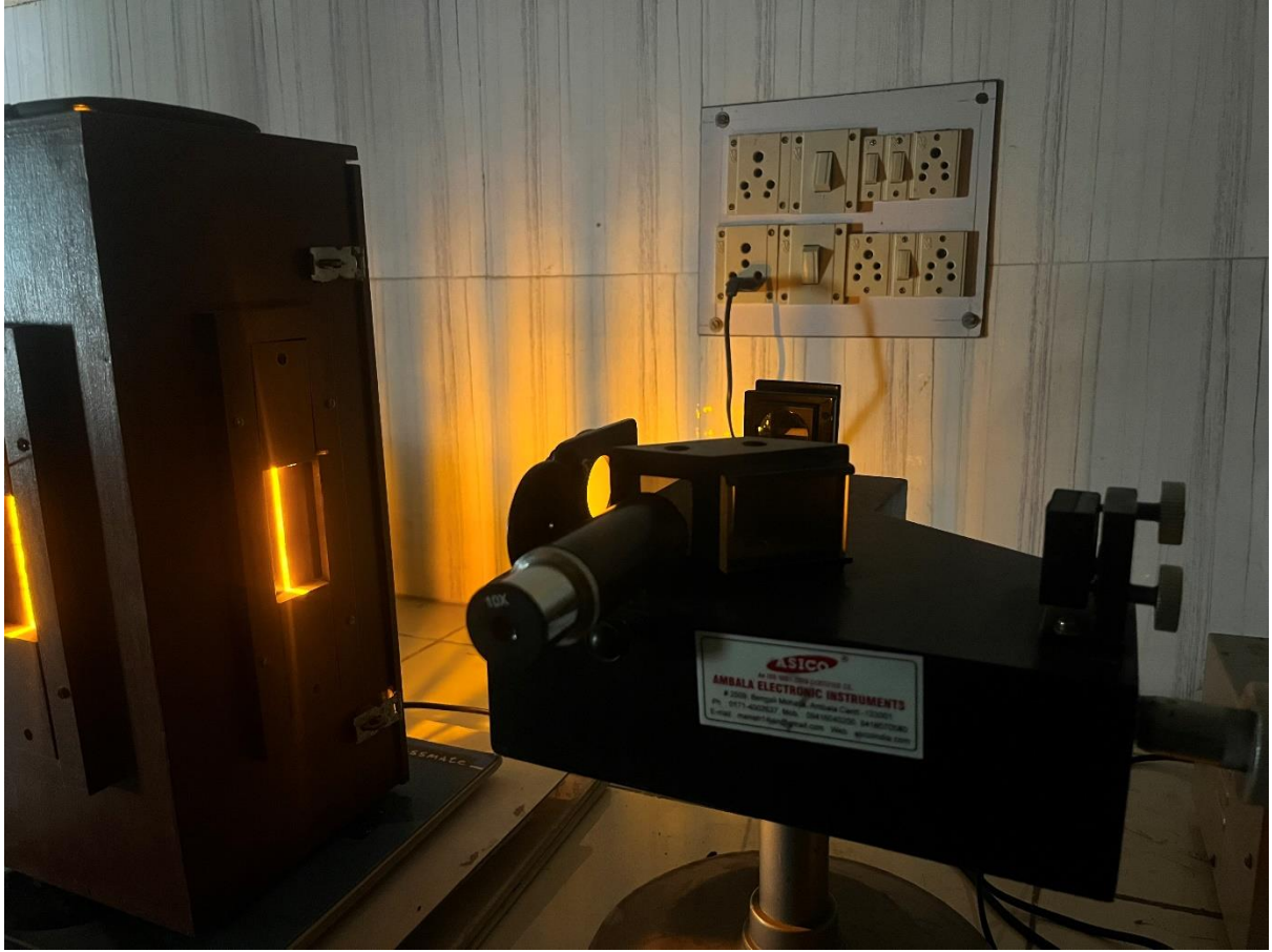
Michelson Interferometer
